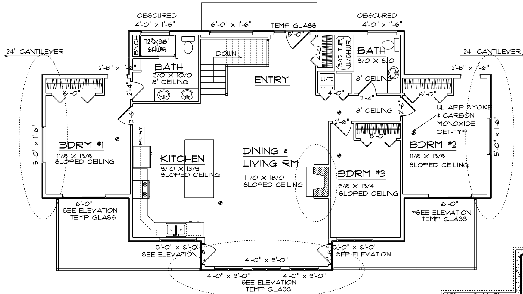
1ST FLOOR LAYOUT SCALE: 1/8" = 1'-0"
